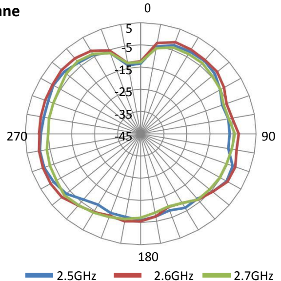
E Plane - 2500 - 2700MHz
