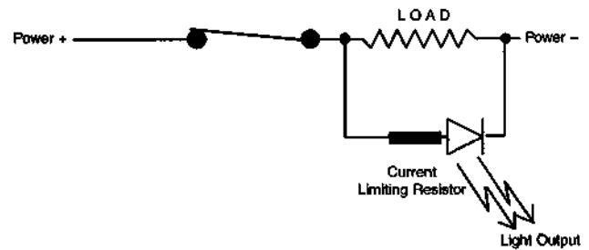
Figure 19. Wiring Diagram 4
