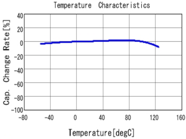
GCM155R71C154KE02 C-Temp. capchange, DC0.0V, AC1.0V rm
