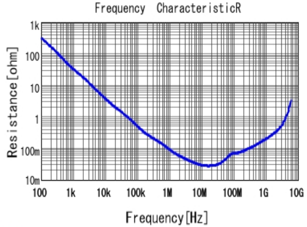
GCM155R71C154KE02 R DCOV, 25degC
