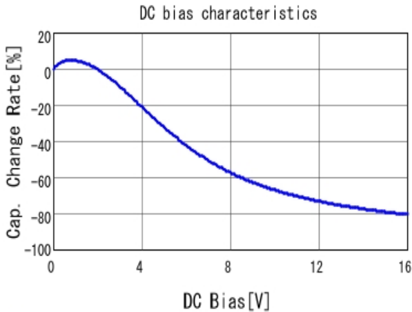
GCM155R71C154KE02 C-DC bias capchange, 25.0degC, AC1.
