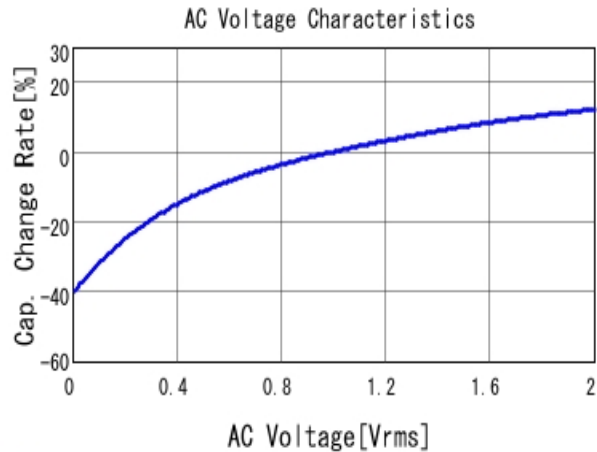
GCM155R71C154KE02 C-AC Voltage capchange, DCOV, 25.0d
