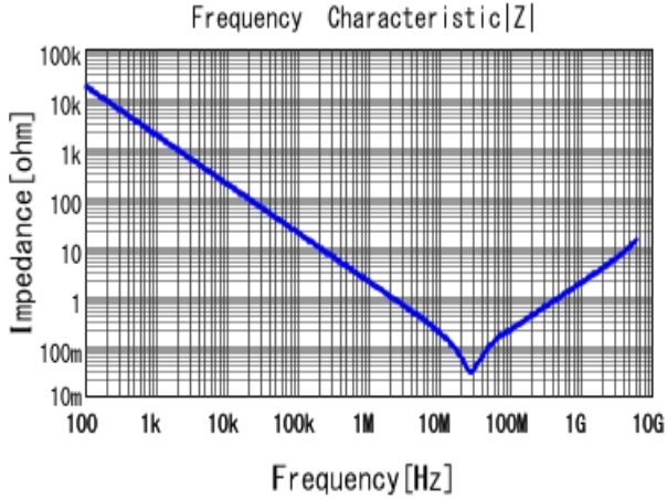
GCM155R71C154KE02 |Z| DCOV, 25degC
