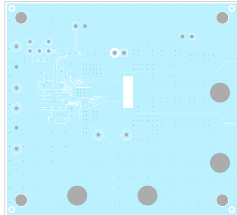
Figure 6. Top Layer
