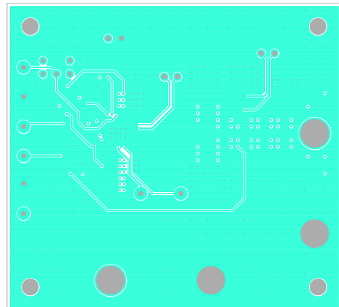
Figure 8. Layer 3
