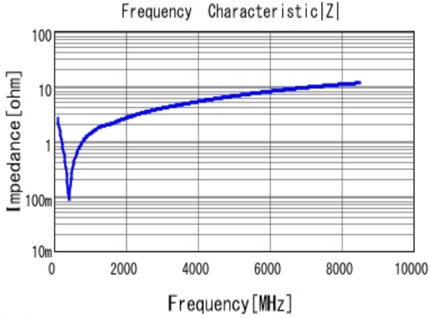
■ GRM0335C1E561JA01 |Z| DC0V, 25degC
