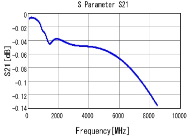
■ GRM0335C1E561JA01 S21 DCOV, 25degC
