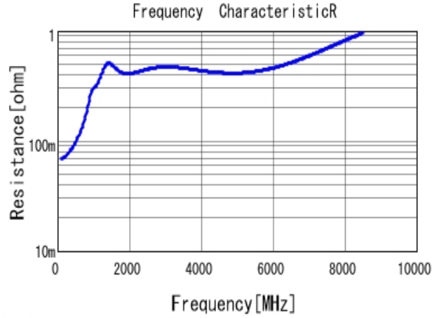
■ GRM0335C1E561JA01 R DC0V, 25degC
