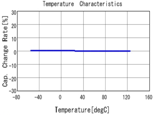
■ GRM0335C1E561JA01 C-Temp. capchange, DCOV, AC1Vrms
