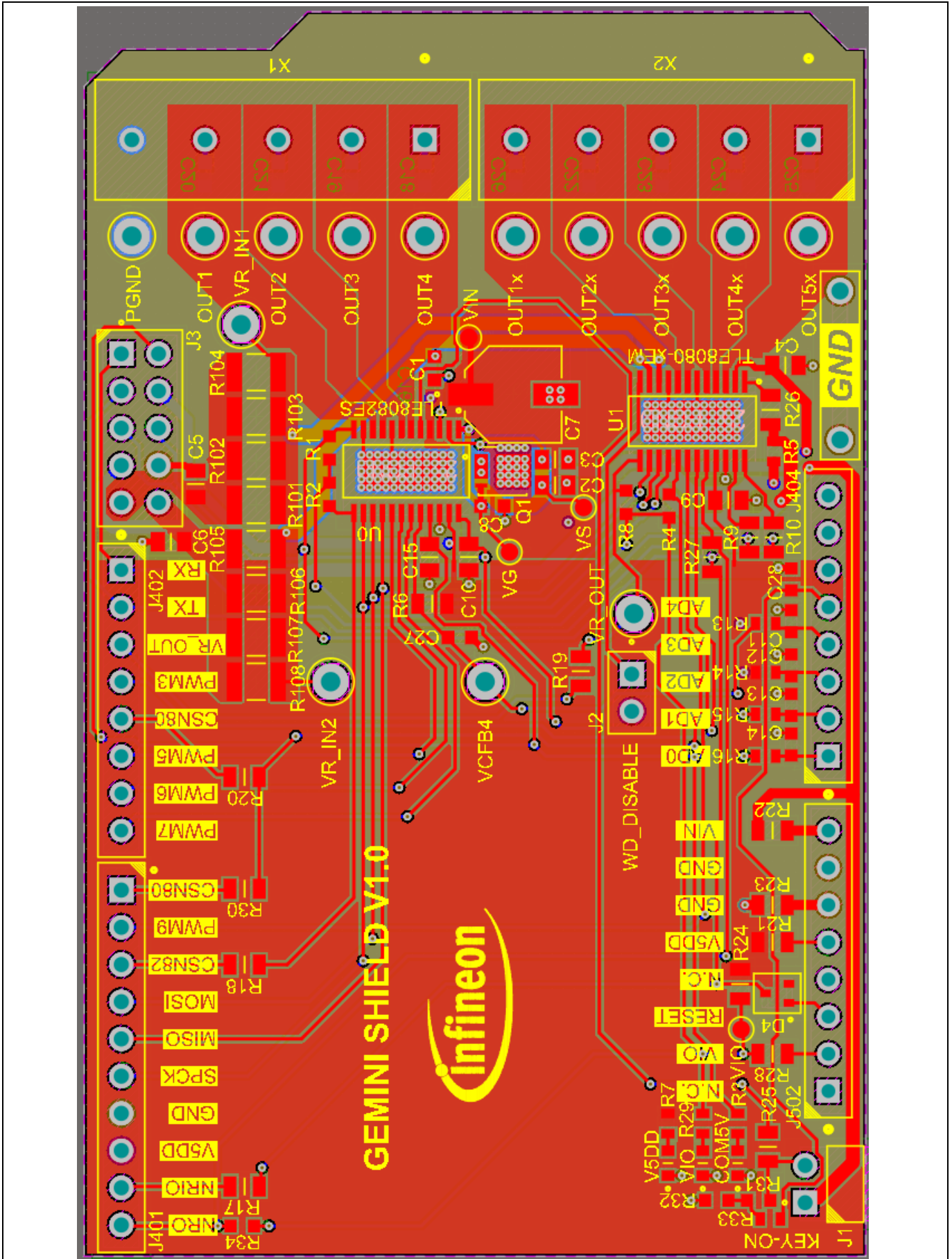
Figure 11 Layout Evaluation-PCB
