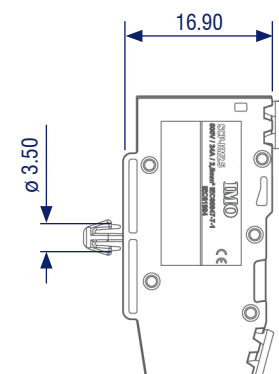
NOTE: Dimensions above are in mm
