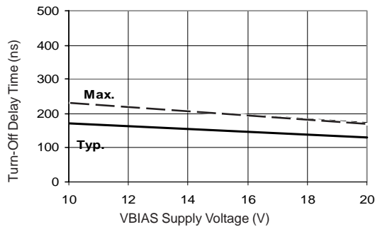
Figure 11B Turn-Off Time vs. Supply Voltage
