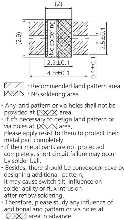
PWB land pattern for reference
