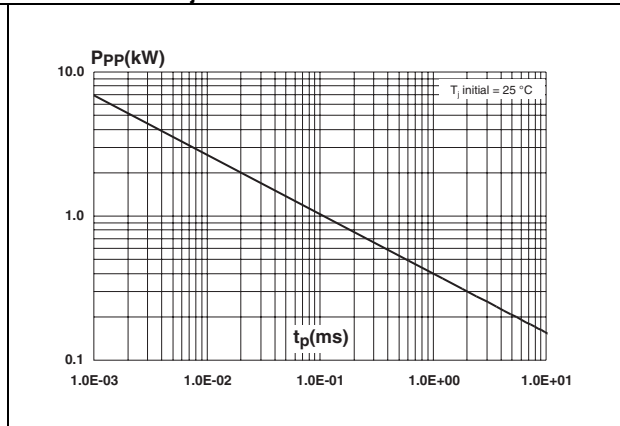
Figure 3. Peak pulse power versus exponential pulse duration (T j initial = 25 °C)
