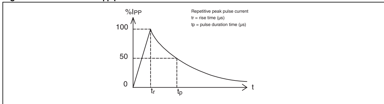
Figure 1. Definition of I_{PP} pulse
