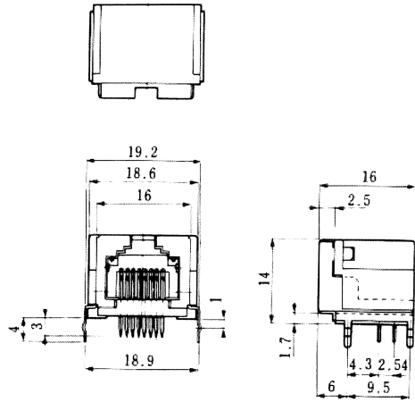
Board mounting dimensional drawing (connector side)
