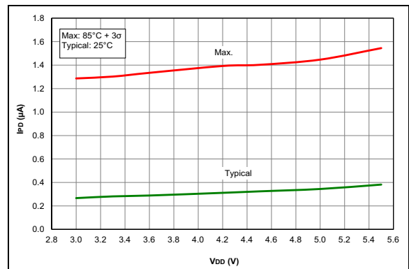
FIGURE 29-30: I_{PD} , LP Brown-Out Reset (LPBOR = 0), PIC12F1612/16F1613 Only.
