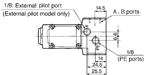
Bottom Ported
