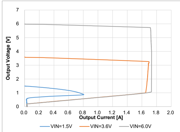
(10-2-2) Output Voltage vs Output Current
