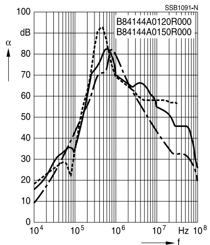
Filters for 120 A and 150 A
