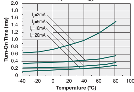
Typical Turn-On Time vs. Temperature ( I_L=120\text{mA}_{\text{DC}} )
