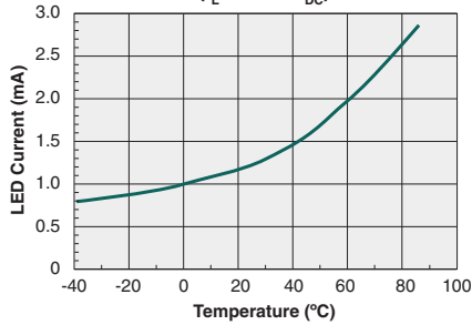
Typical I_F for Switch Operation vs. Temperature ( I_L=120\text{mA}_{\text{DC}} )
