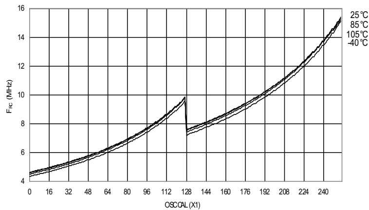
Figure 30-38. Calibrated 8MHz RC Oscillator vs. OSCAL Value
