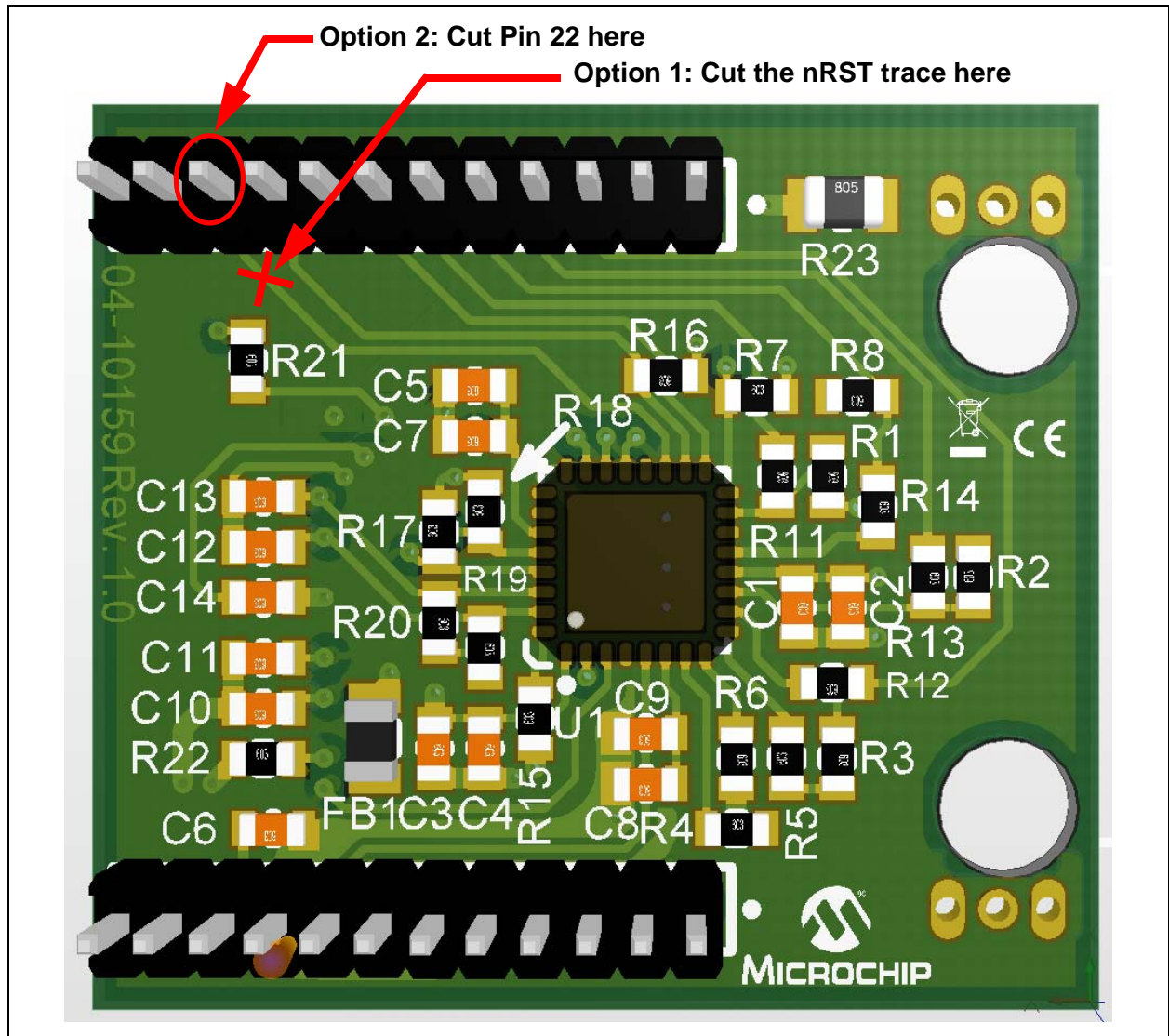
FIGURE 1: LAN8740 PHY DAUGHTER BOARD LAYOUT
