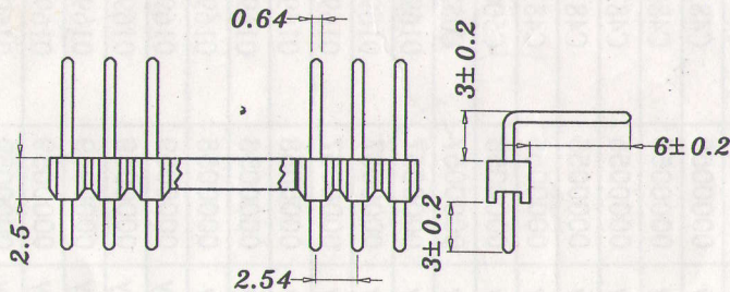
Single Row-Right Angle Pins
