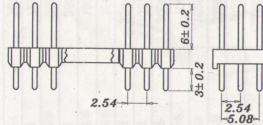
Double Row-Straight Pins
