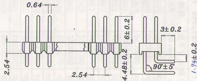
Double Row-Right Angle pins
