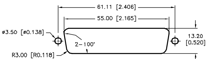
PANEL CUTOUT
