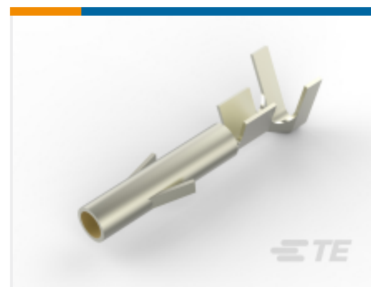
TE Part # 350551-7 UMNL SOK 20-14 AU/BR L/P
