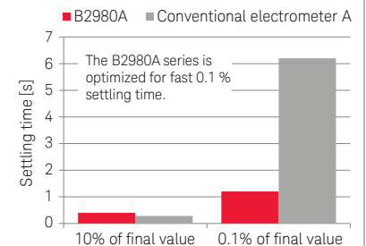
20 pA range settling time 2 V step, 100 GΩ, 1 PLC
