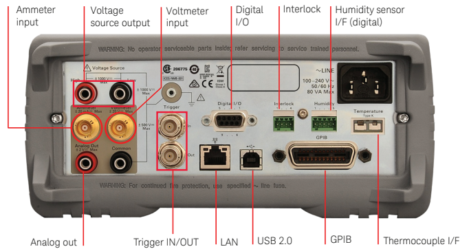
B2985A, B2987A Electrometer/High Resistance Meter
