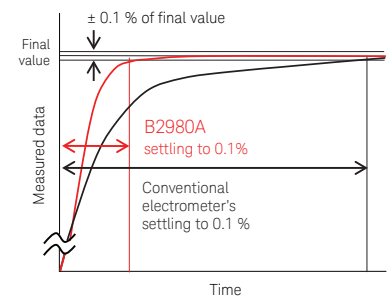
20 pA range settling time 2 V step, 100 GΩ, 1 PLC
