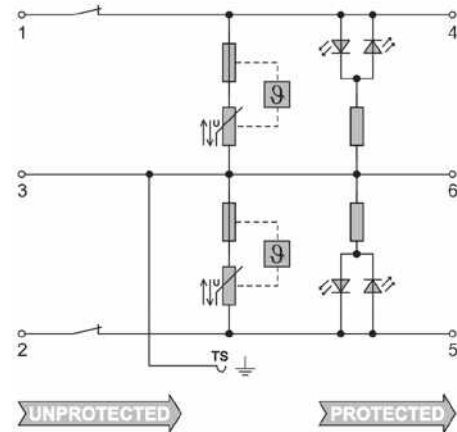
Circuit diagram
