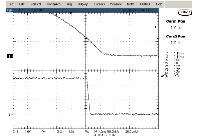
Figure 18: Remote turn off delay time at 24vin, 2.5V/3A out
