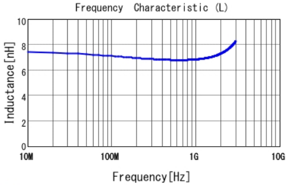
■ LQP03TN6N8H02 L
