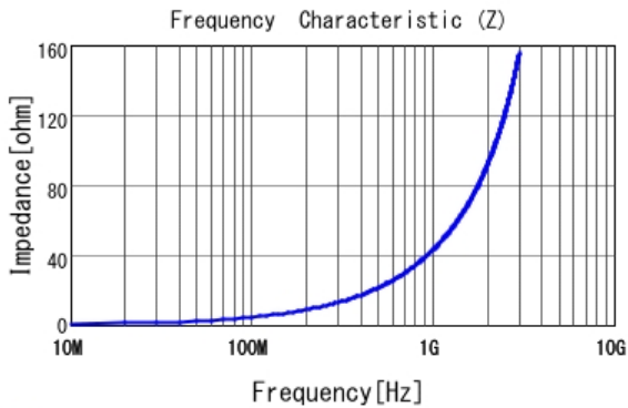
■ LQP03TN6N8H02 |Z|
