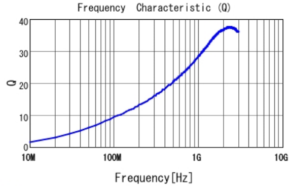
■ LQP03TN6N8H02 Q
