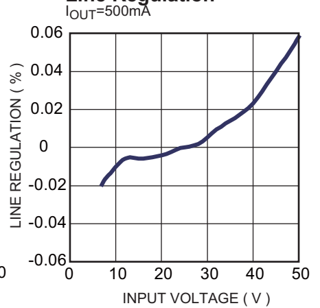
Line Regulation
