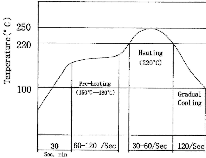
ABT-425-RC Reflow Soldering Curve
