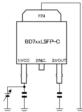
TO252-3
