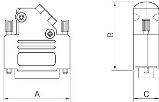
D-Sub-Hood
