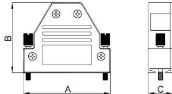
D-Sub-Hood
