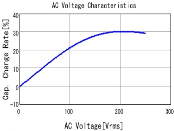
■ DE2E3SA222MN3AT02F C-AC Voltage capchange, DCOV, 20.0
