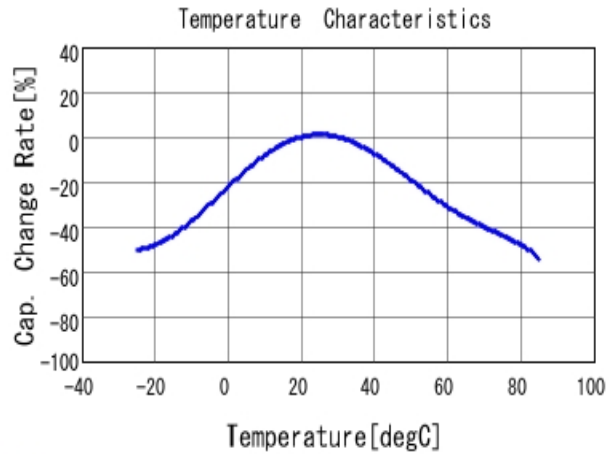
■ DE2E3SA222MN3AT02F C-Temp. capchange, DCOV, AC1Vrms
