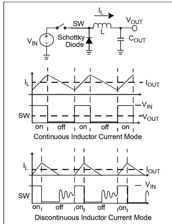
FIGURE 5-1: Step-Down Converter.
