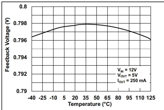
FIGURE 2-8: V_{FB} vs. Temperature.
