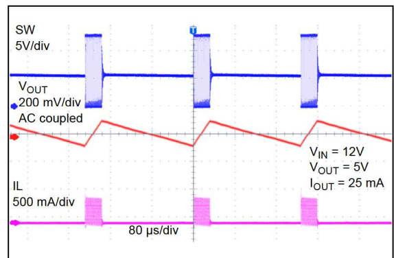
FIGURE 2-24: Light Load Switching Waveforms – MCP16361.
