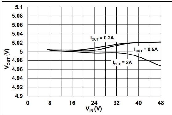
FIGURE 2-7: V_{OUT} vs. V_{IN} .
