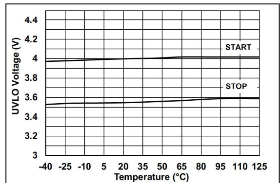
FIGURE 2-12: Undervoltage Lockout vs. Temperature.
