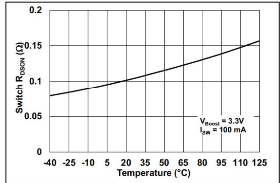
FIGURE 2-10: Switch R_{DS(on)} vs. Temperature.
