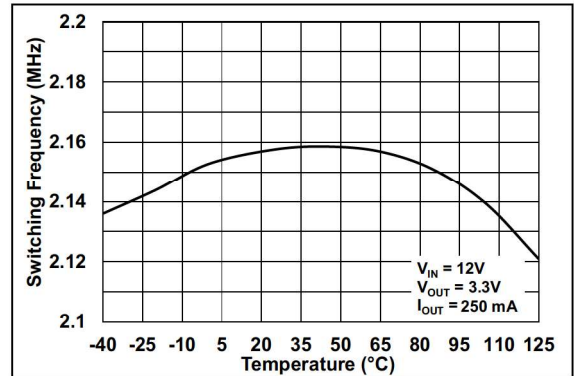
FIGURE 2-22: Switching Frequency vs. Temperature.
