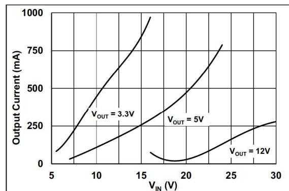
FIGURE 2-18: PFM/PWM Threshold.
