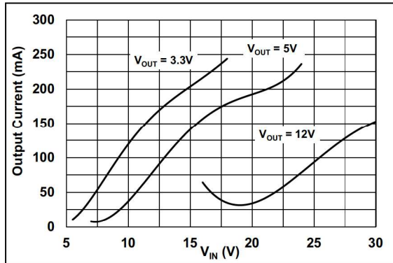
FIGURE 2-19: PWM/Skipping Threshold.
