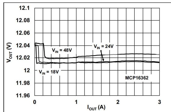
FIGURE 2-6: 12V V_{OUT} vs. I_{OUT} .
