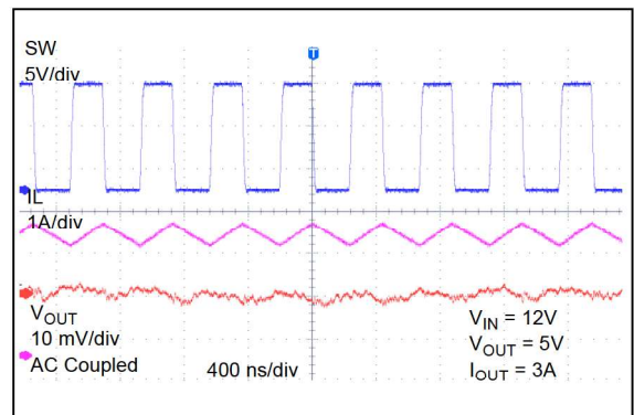
FIGURE 2-23: Heavy Load Switching Waveforms.
