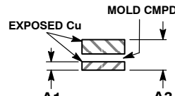
DETAIL B ALTERNATE CONSTRUCTION
