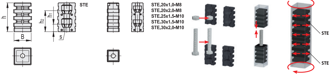
The geometry of the end-cap in the part that is inserted into the tube may vary for the different dimensions.
