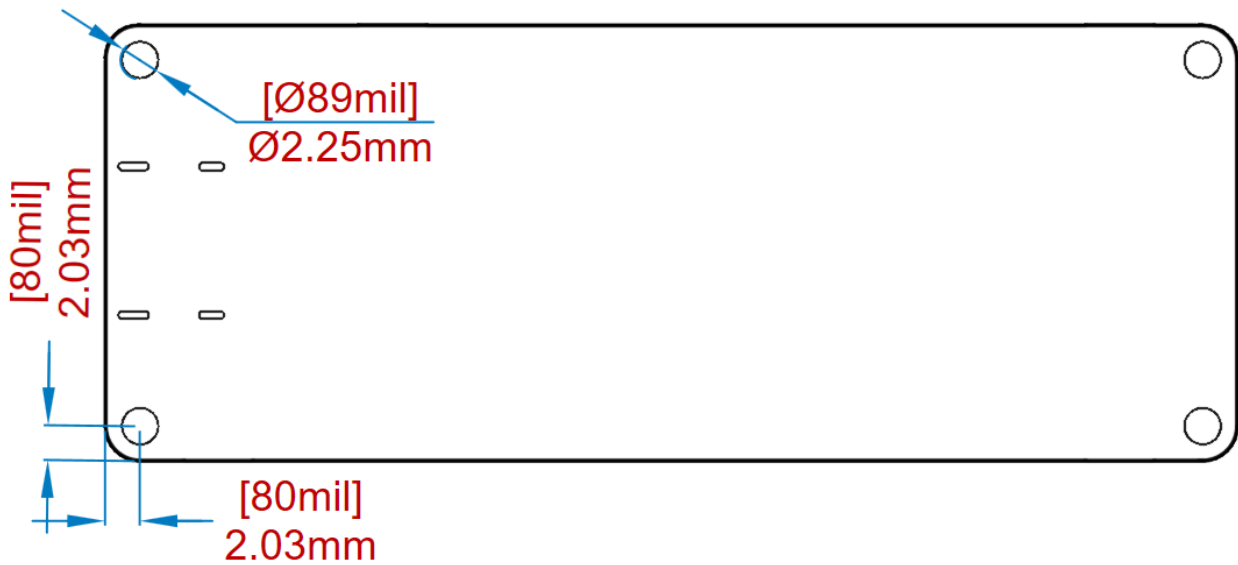
Mounting outline
