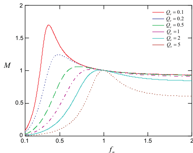
Figure 16. Normalized Switching Frequency vs. Converter Voltage Gain, L_n=10
