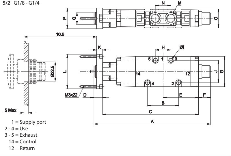
5/2 G1/8 - G1/4
