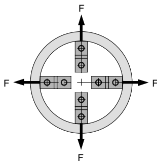
Internal gripping
