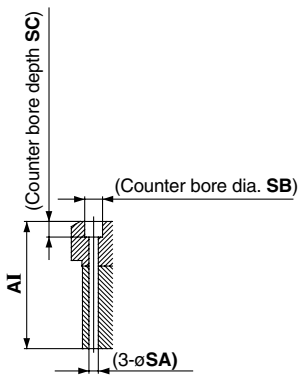
Section SD - SD
