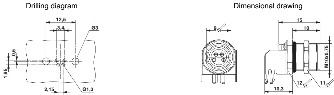
M8 flush-type socket
