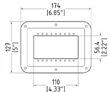
Large Dish, punched for 2.5 Modules of 2 Unit MSB front panes.
