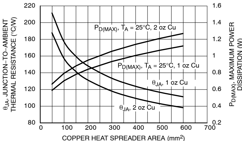
Figure 66. \theta_{JA} and P_{D(\text{MAX})} vs. Copper Area (WDFN6)
