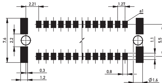
Recommended Layout
