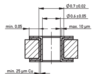
Hole Design
