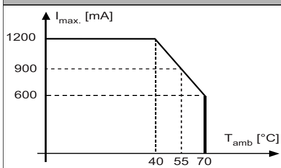
(2) BWU1938, BWU2721, BWU2723, BWU2759 Derating power supply of attached sensors
