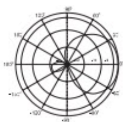
V-Plane Co-polarization Pattern
