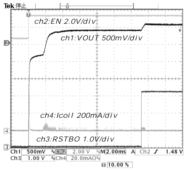
Figure 25. RISE [EN : OFF=>ON] PFM VIN=3.2V Io=0mA
