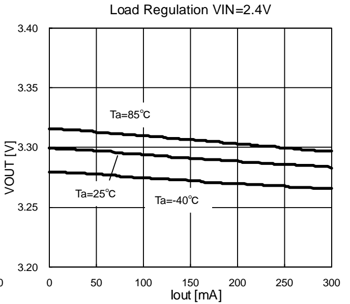
Figure 17. Load Regulation PWM VIN=2.4V
