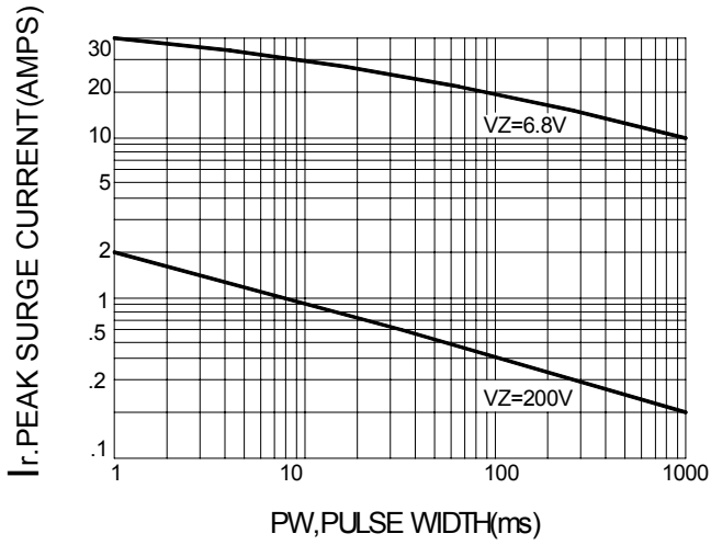
FIG.6 – PEAK SURGE CURRENT VERSUS PULSE WIDTH
