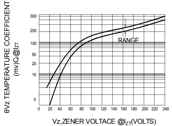
FIG.2 -- TEMPERATURE COEFFICIENT RANGE
