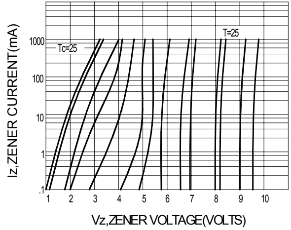
FIG.7 – ZENER VOLTAGE VERSUS ZENER CURRENT Vz=6.8 THRU 10 VOLTS
