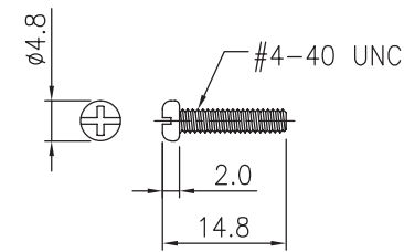
SCREW 2PCS
