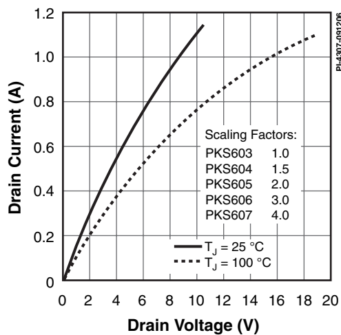
Figure 26. Output Characteristic.
