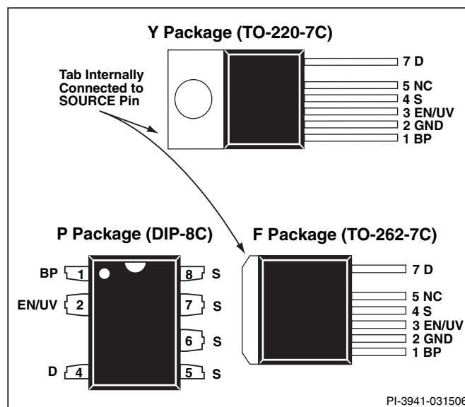
Figure 3. Pin Configuration.
