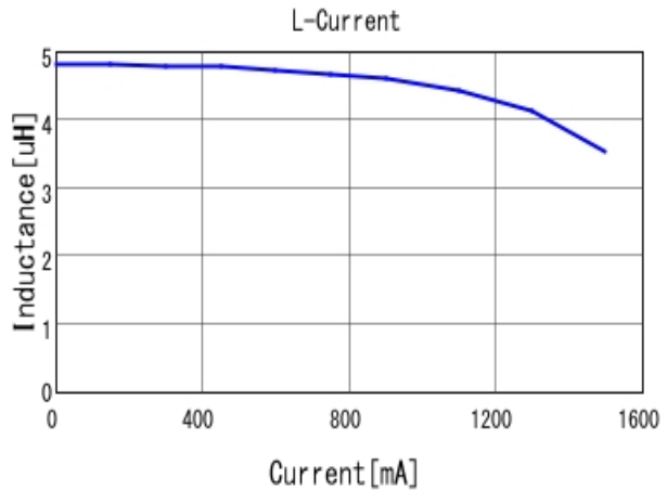
#A914BYW-4R7M=P3 L-Current 20degC
