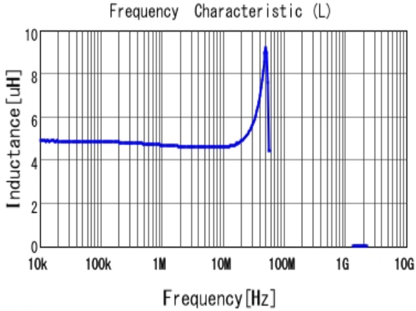
#A914BYW-4R7M=P3 L
