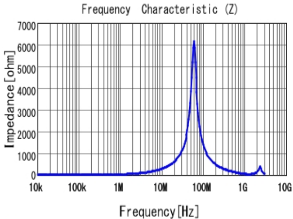
#A914BYW-4R7M=P3 |Z|
