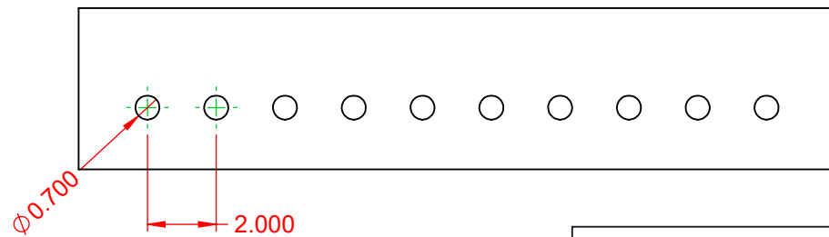
SUGGESTED PCB LAYOUT
